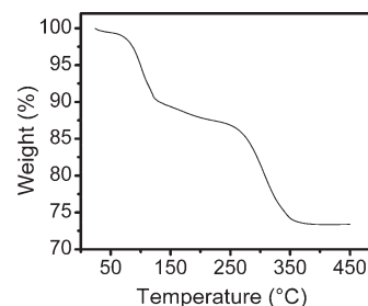
Figure 2. TGA data of a CIS precursor ( 1\text{ }^\circ\text{C}/\text{min} ramp; \text{N}_2 atmosphere).
